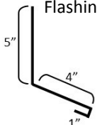
Apron or Side Wall Flashing
