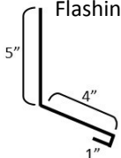
Apron or Side Wall Flashing
