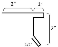
Apron or Side Wall Flashing
