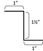
Standard Under Siding Counter Flashing
