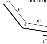
Standard 1" Z Bar
